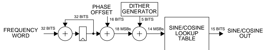
Figure 4. NCO Circuit
